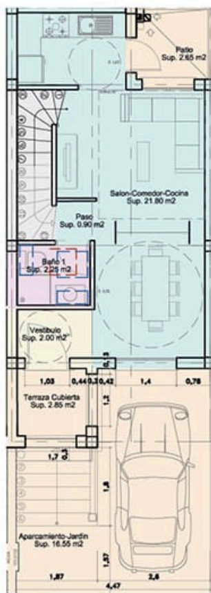
PLANTA BAJA GROUND FLOOR
